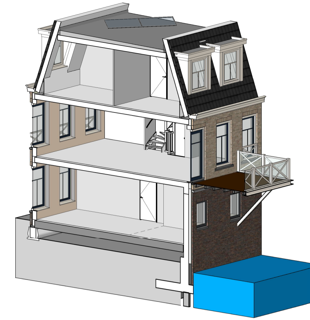
3D impressie
