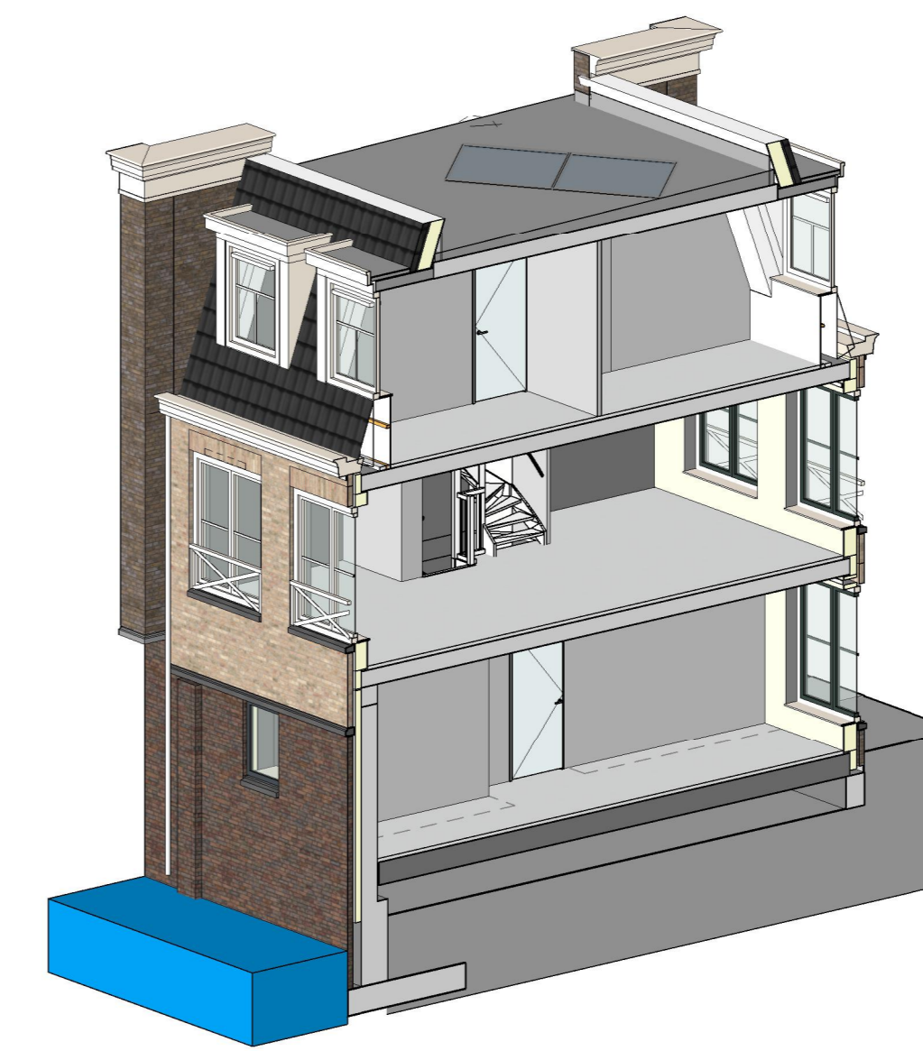
3D impressie
