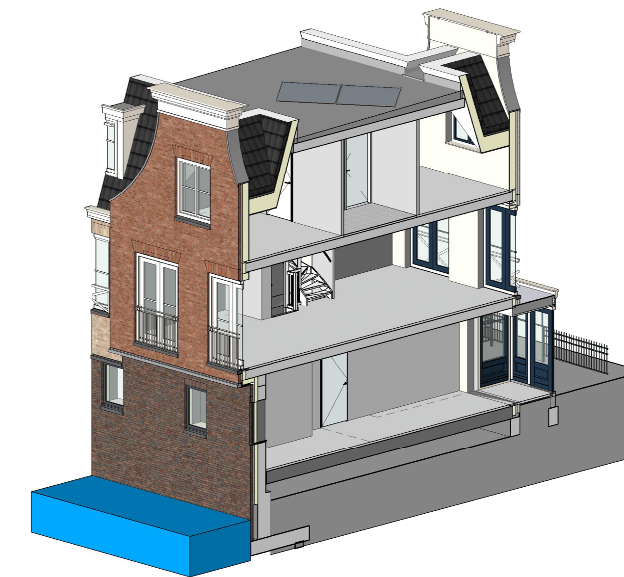
3D impressie
